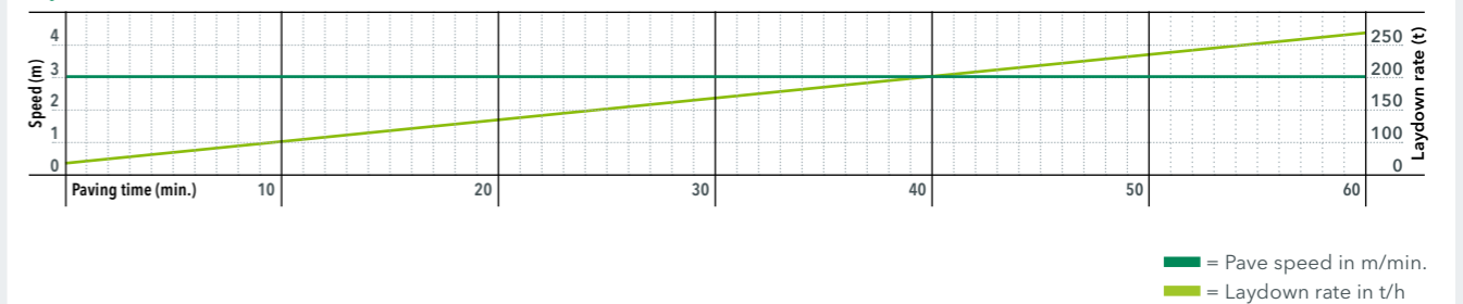
Operation with a VÖGELE PowerFeeder (in m/min.)
